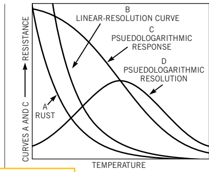
Figure 1 These resistance-versus-temperature curves highlight the improved resolution available in a pseudologarithmic circuit.
