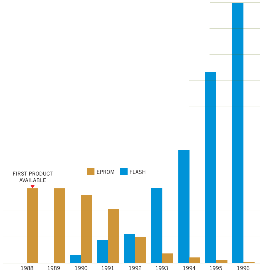
Figure 1 Within five years, NOR flash-memory shipments had surpassed those of EPROM; EPROM soon faded away (courtesy Intel).
