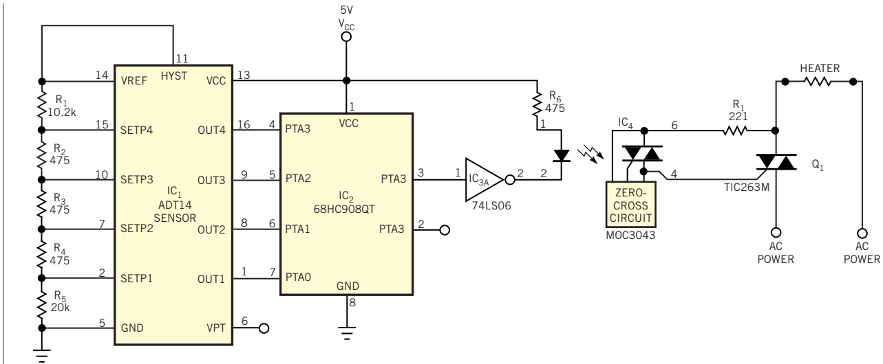
Figure 1 This proportional temperature controller features a minimal parts count.
