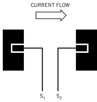
Figure 2 Modified pads provide isolated Kelvin connections that eliminate errors introduced by voltage drops across soldered connections carrying high current.
