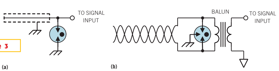
Single- (a) and triple-pole (b) gas-discharge tubes protect coaxial and balanced twisted pairs.
