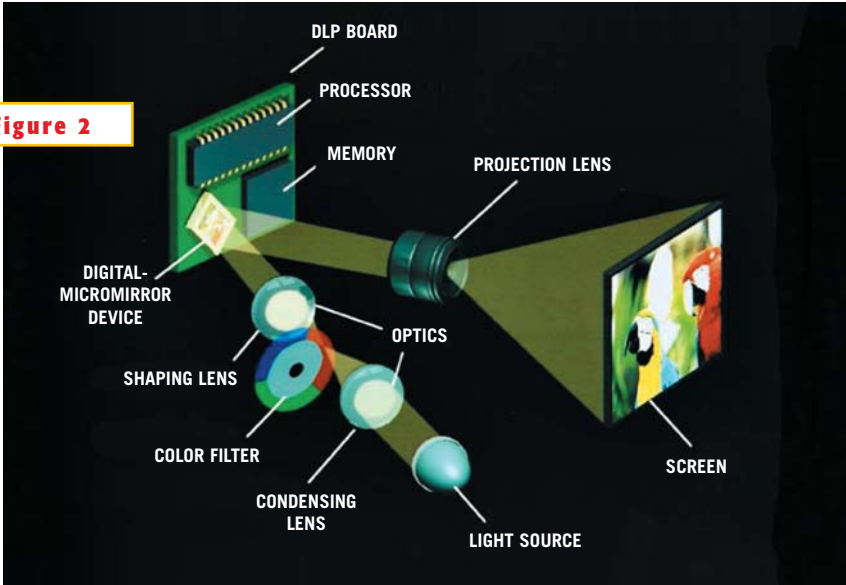
TI's DLP (digital-light-processor) microdisplay allows a single device to project all three colors of an image sequentially, eliminating the need for pixel alignment (courtesy Texas Instruments).
