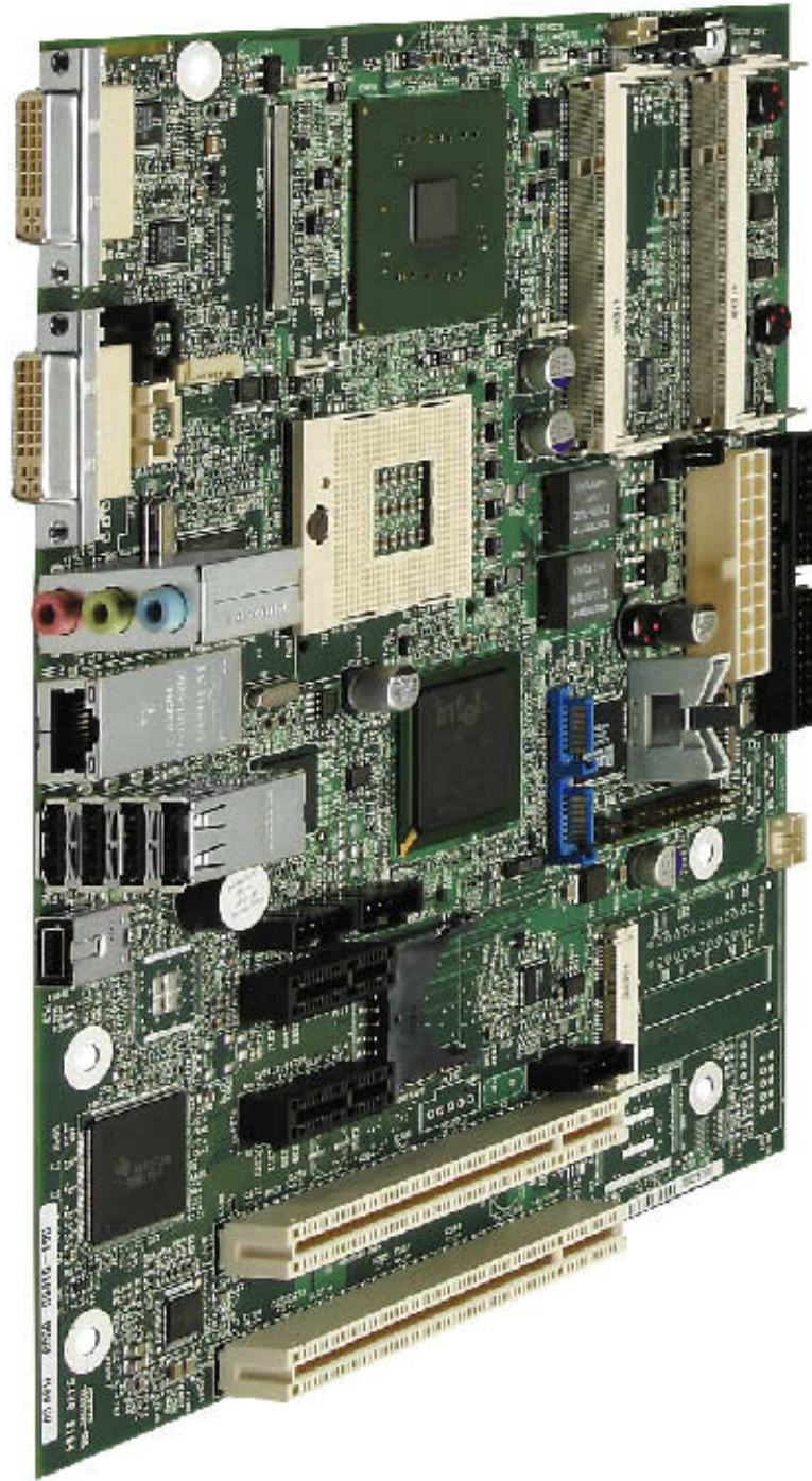
RadiSys' new Endura AB915GM motherboard provides both PCI and PCI Express slots and a PCI Express Mini Card slot.
