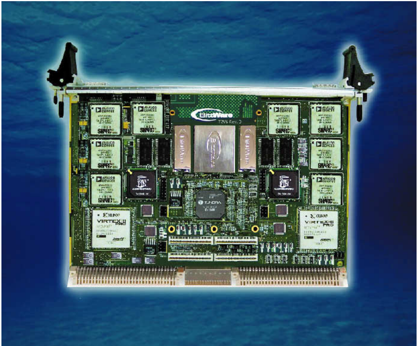
Available in both convection- and conduction-cooled versions, BittWare's T2-6U-VME features eight 600-MHz TigerSHARC DSPs and two Xilinx FPGAs.
