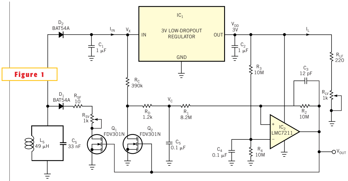
A low-power VFC and load modulator measure power generated by a wireless-telemetry power source.
