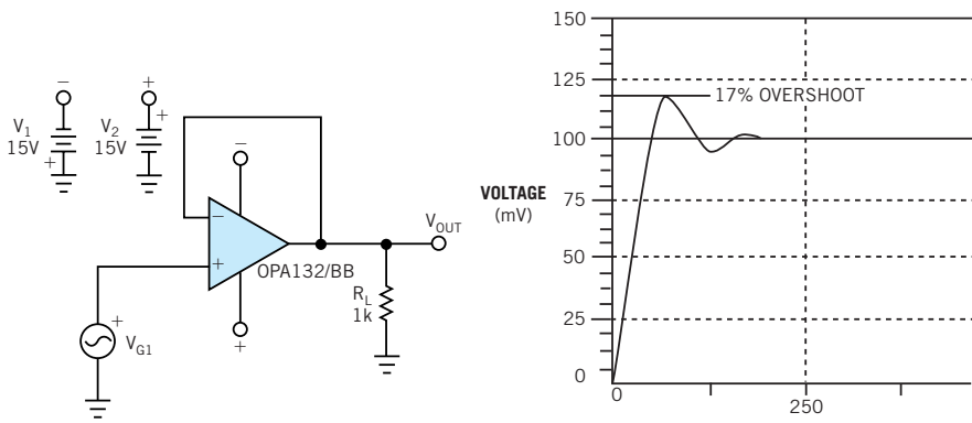
Figure 3 The step response of the op amp correlates with the 50^\circ phase shift.
