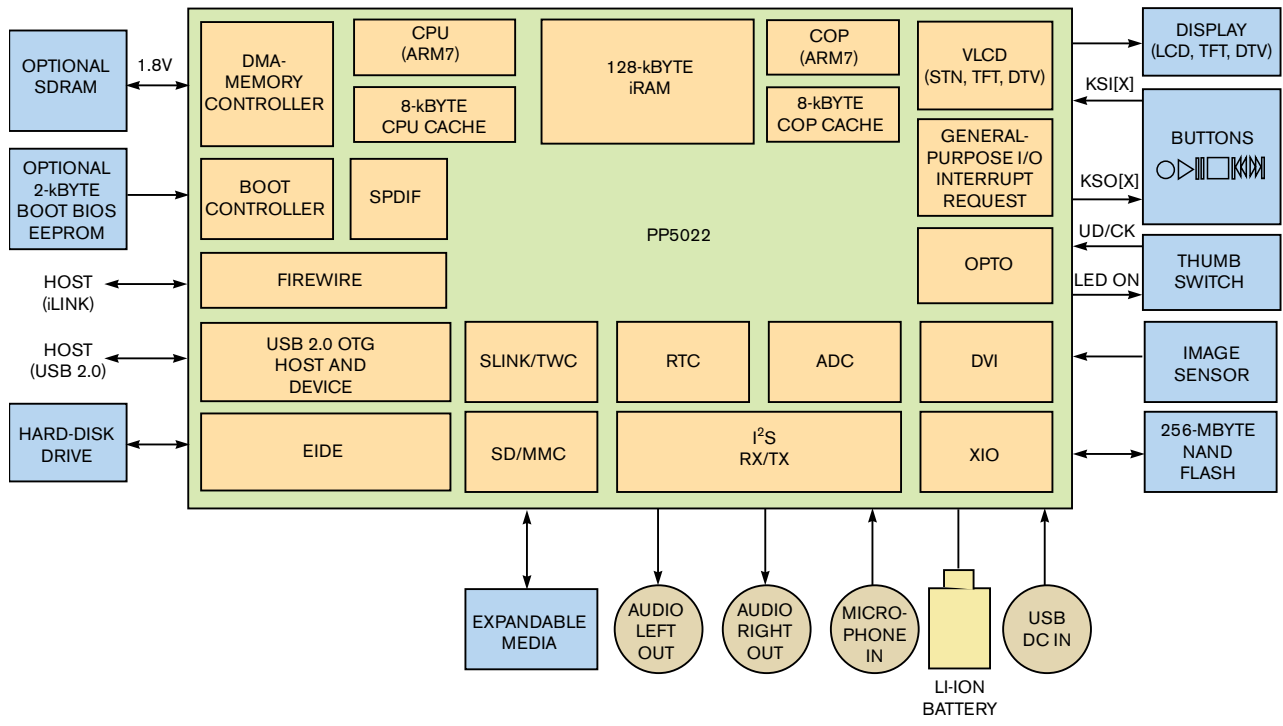
Figure 4 The highly integrated PortalPlayer PP5022's use of a low-current, 0.13-micron process leads to significant power savings.
