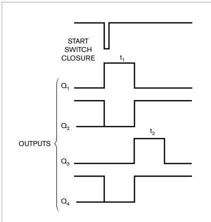
Figure 2 This timing diagram illustrates outputs available from the timer's two sections.
