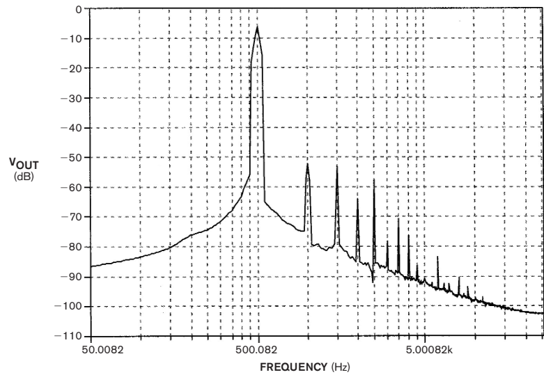
Figure 2 The oscillator's output spectrum contains second- and third-harmonic levels of at least 250 dB below the fundamental.
