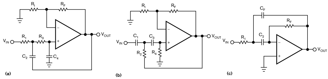
Figure 1 The Sallen Key lowpass filter (a), highpass filter (b), and multiple-pass filter (c) each require only one op amp.
