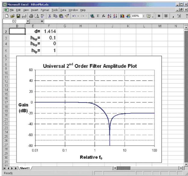
Figure 8 The highpass and lowpass coefficients, along with f_0 , determine that the response is zero.
