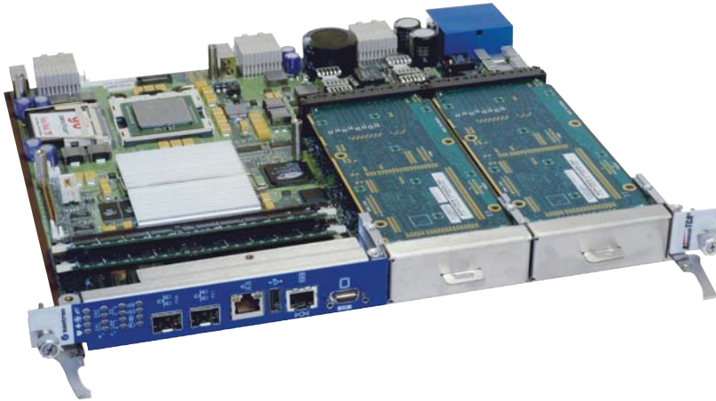
Figure 2 The AT8001 server blade from Kontron is one of the first AdvancedTCA boards to support the AMC.0 and AMC.1 specifications and offers space for two AdvancedMC modules.
