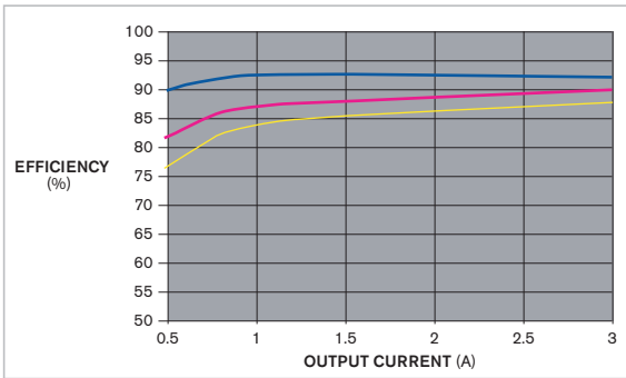
Figure 2 Circuit efficiency varies as functions of power-supply input voltage and load current.
