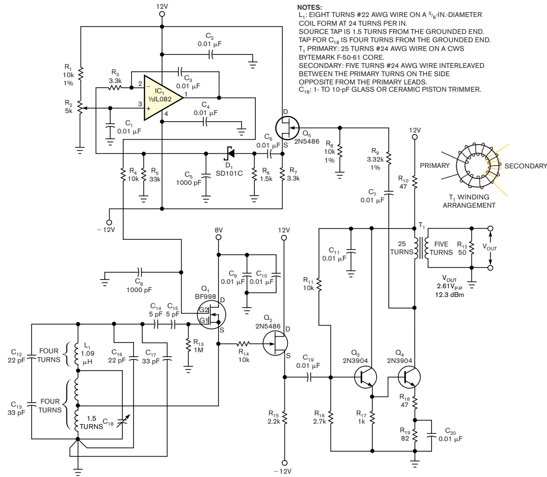
Figure 1 This low-distortion, 18-MHz oscillator offers high stability and automatic output-level control.
