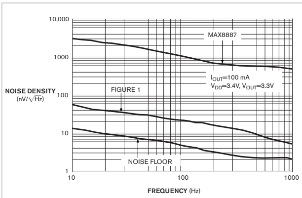
Figure 3 A noise-density-versus-frequency plot for the low-dropout circuit in Figure 1 is 38 dB lower than that of a conventional low-noise, low-dropout-voltage regulator—in this case, a Maxim MAX8887.
