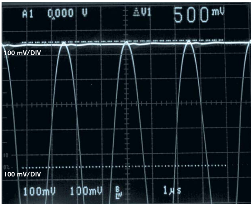
Figure 3 An oscilloscope photo displays input versus output voltages for a 400-kHz, 500-mV sine wave.
