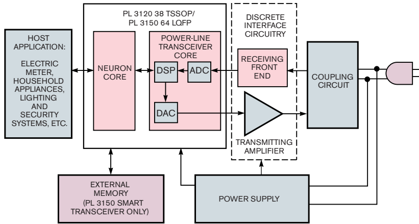
Figure 3 Echelon's smart power-line transceivers enable LonWorks-compatible products to communicate over a building's electrical network.
