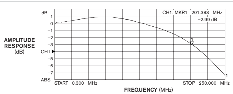
Figure 2 The probe's measured -3 -dB frequency response extends from 10 Hz to 200 MHz with slightly less than 1-dB passband ripple, which compares favorably with the \pm 2 -dB response of many commercial active-FET probes.
