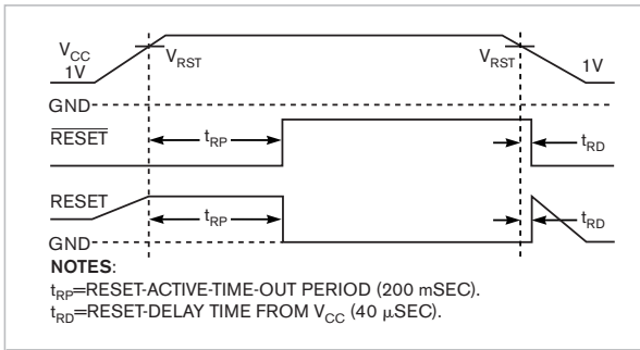
Figure 3 Reset-timing relationships for the circuit of Figure 2 illustrates its power-on behavior.
