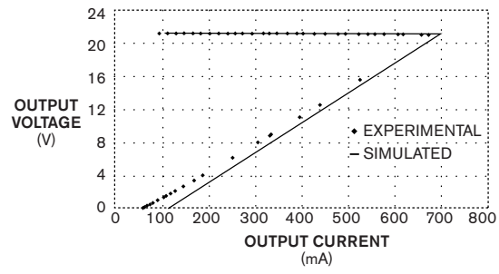
Figure 2 Simulated and measured foldback-current responses to a load resistance that varies from 200 to 0.01\ \Omega show close agreement.
