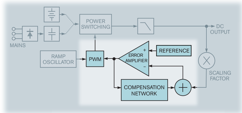
Figure 1 An analog SMPS control loop compares a scaled sample of the output voltage with a fixed reference and servos the PWM timing to force the two quantities to match.
