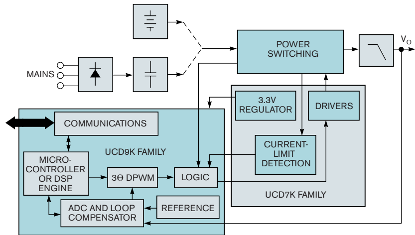
Figure 4 Texas Instruments' UCD9k and UCD7k ICs combine to form a digital power controller.
