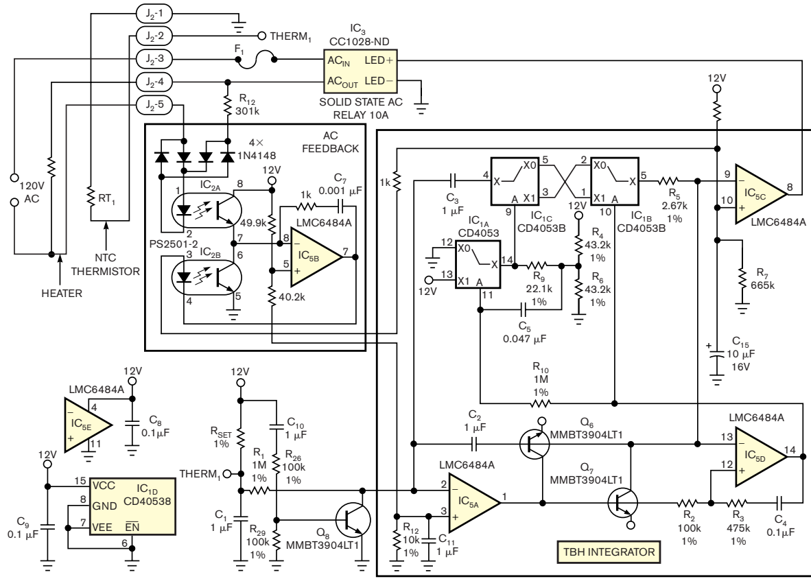
Figure 3 For safety, this version of a TBH heater controller features full isolation of the ac-line and control circuits.
