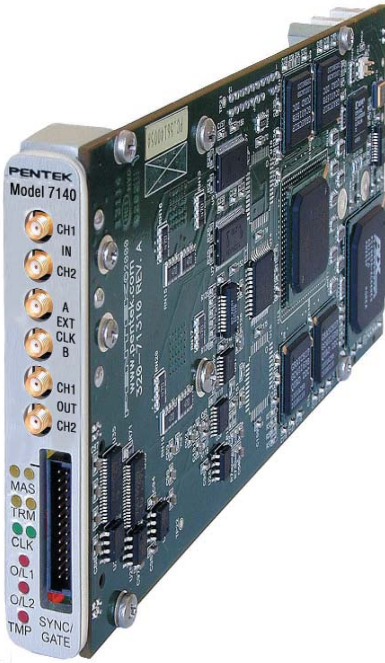
Figure 3 The Model 7140 PMC module from Pentek combines digital-radio transceivers with a Virtex II-Pro FPGA with room for user-defined DSP functions.
