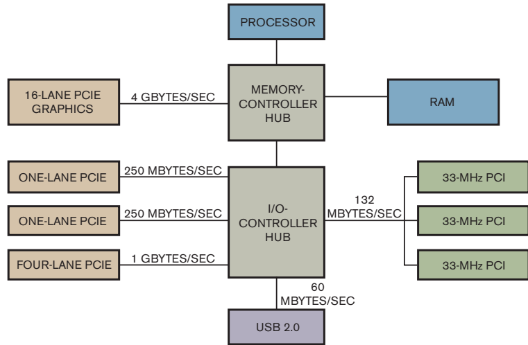
Figure 1 Each PCI Express slot has dedicated bandwidth to memory, unlike PCI, which shares bandwidth.
