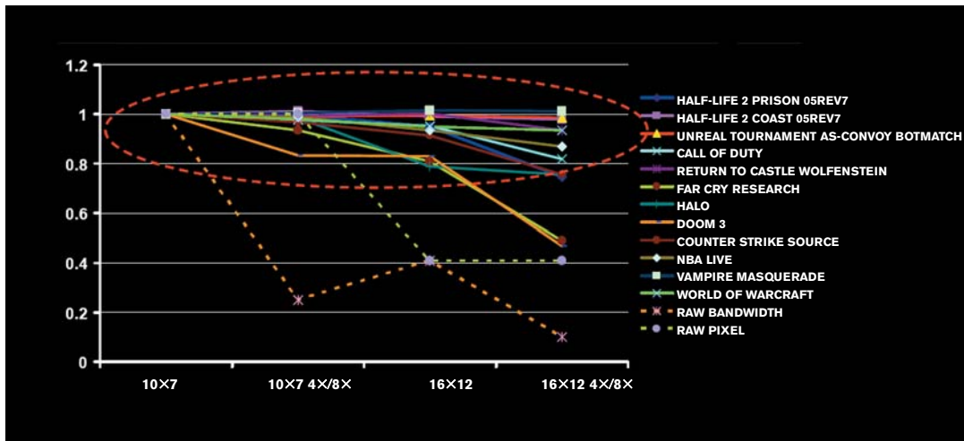
Figure 1 Minor to nonexistent decreases in frame rates with increasing graphics complexity suggest that the CPU, not the GPU, is the performance bottleneck (courtesy Nvidia).
