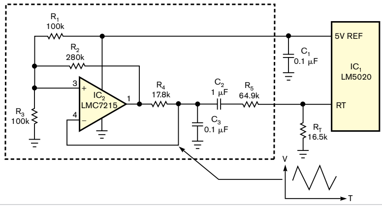
Figure 1 A low-frequency triangular-wave oscillator modulates a PWM controller's oscillator frequency.
