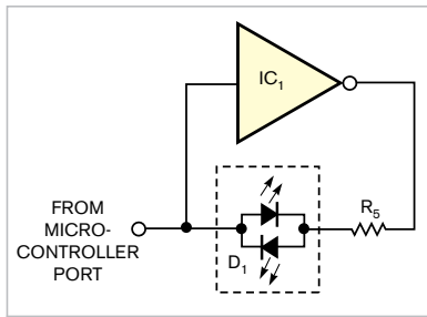
Figure 1 An inverter can drive a bidirectional, two-color LED but applies the same amount of current to both LEDs.
