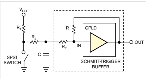
Figure 5 Use a Schmitt trigger to debounce switch contacts.
