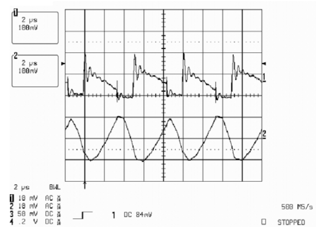
(a) Figure 10 The output-ripple voltage (upper traces in (a) and (b)) illustrates several points. For example, the higher frequency of the interleaved converter's ripple current eases filtering.
