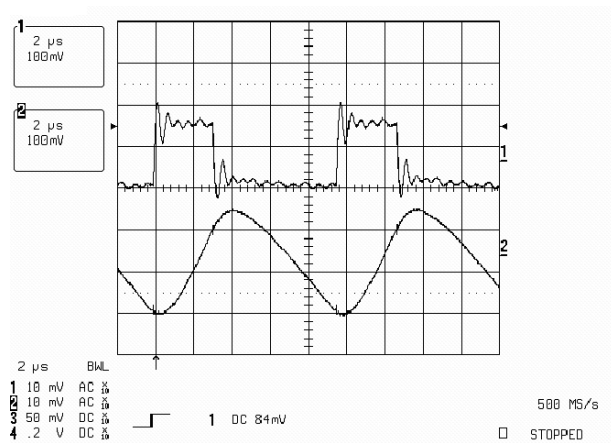
(a) Figure 10 The output-ripple voltage (upper traces in (a) and (b)) illustrates several points. For example, the higher frequency of the interleaved converter's ripple current eases filtering.
