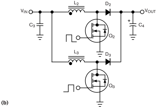
Figure 2 The single-phase supply (a) is simpler than the interleaved-boost supply (b).
