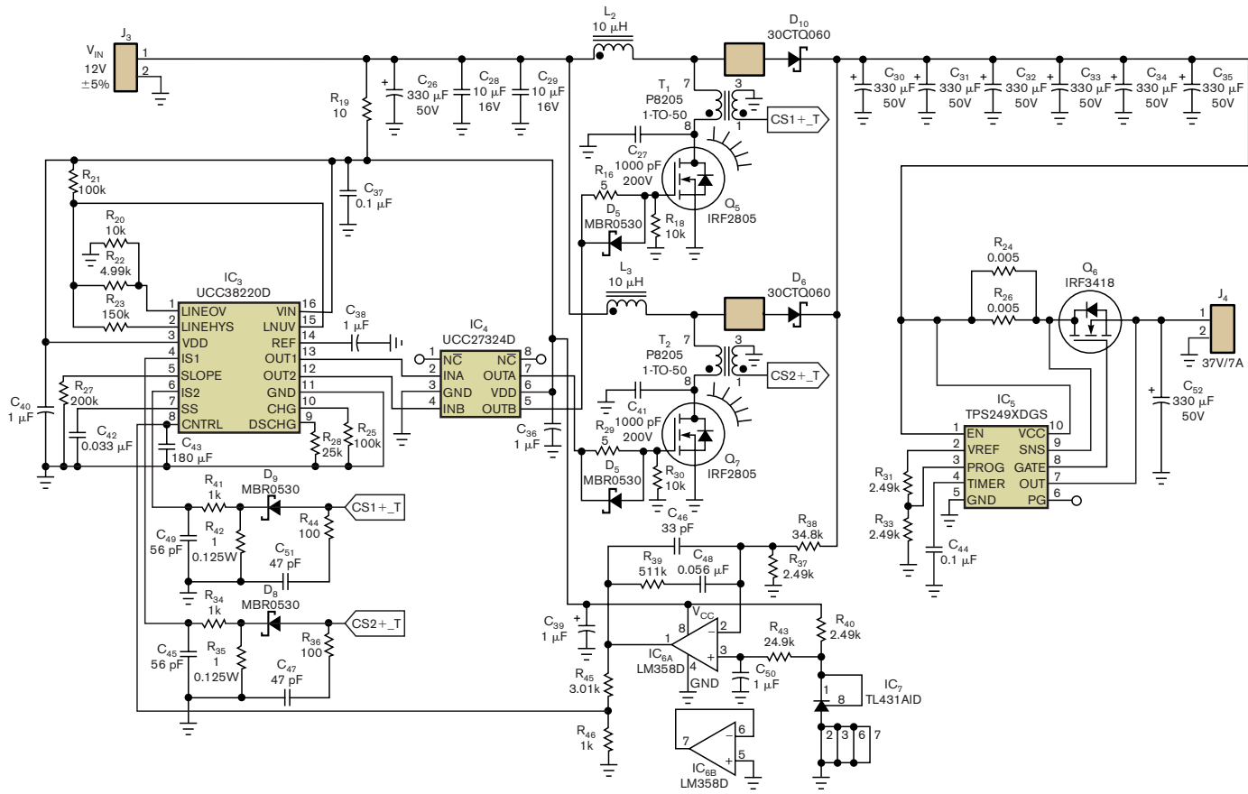
Figure 8 This interleaved design halves the output-capacitor requirements.
