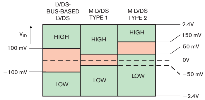
Figure 1 A comparison of receiver threshold voltages shows the differences among various technologies.
