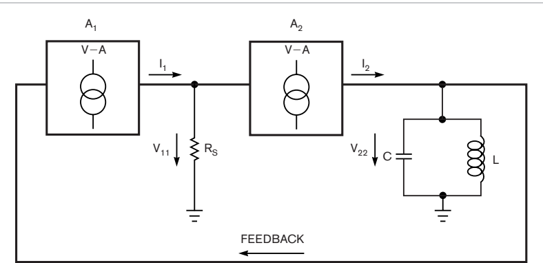
Figure 2 Adding a second voltage-to-current converter isolates the tuned circuit.
