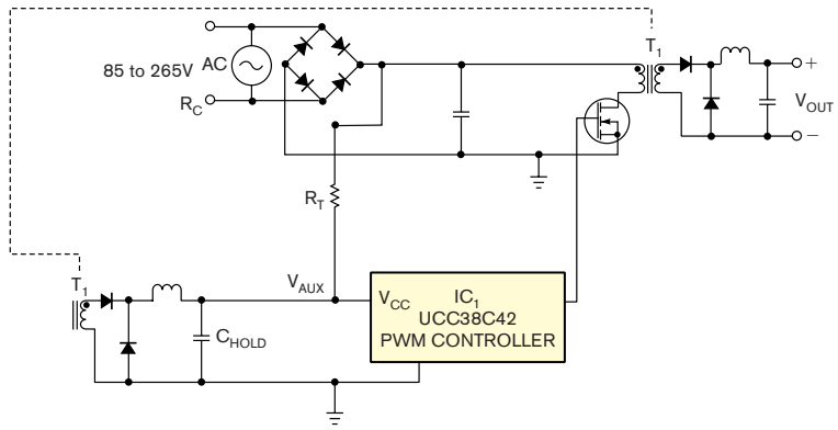
Figure 2 An auxiliary winding supplies power to the supply's PWM controller.
