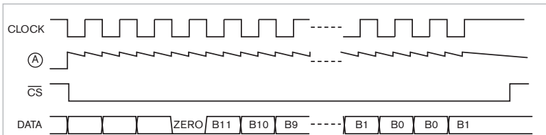
Figure 2 An SPI-clock waveform (top trace) evokes data (bottom trace), and peak detection of the clock (the waveform at Point A in Figure 1) yields a signal (next-to-bottom trace) that mimics the chip-selection line's behavior.
