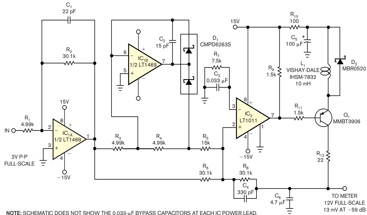
Figure 1 This inductor-compensated voltage-unit meter displays a 60-dB dynamic range.
