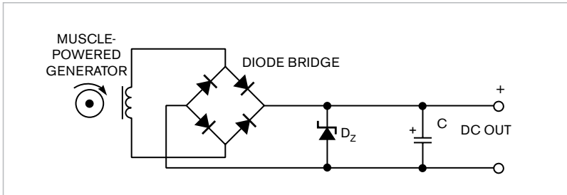
Figure 1 This charger circuit for storage capacitor C requires few additional components: a diode-bridge rectifier and an overvoltage-limiting zener diode.
