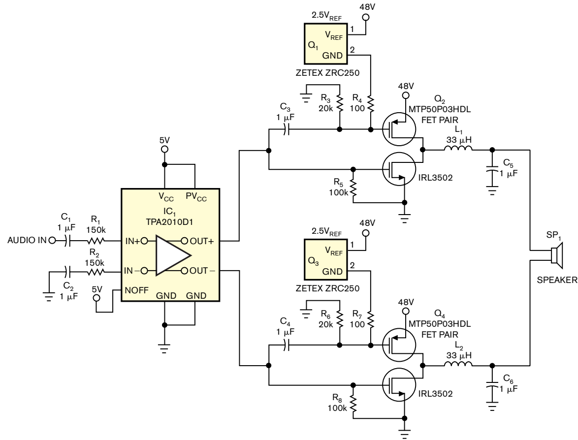
Figure 5 This Class D audio amplifier boosts its driver's output to 200W rms for a 48V power supply.
