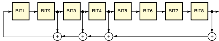
Figure 2 A linear-feedback-shift register generates a pseudorandom bit sequence.
