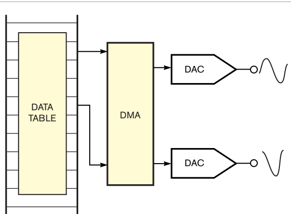
Figure 1 Using DMA, tabulated data values on their way to waveform-generating DACs avoid handling by a system's processor.
