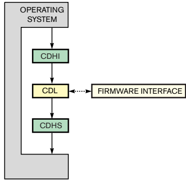
Figure 1 The OS-dependent portion of a CDL divides into the CDHI (common-driver-host-interface) and CDHS (common-driver-host-services) layers.
