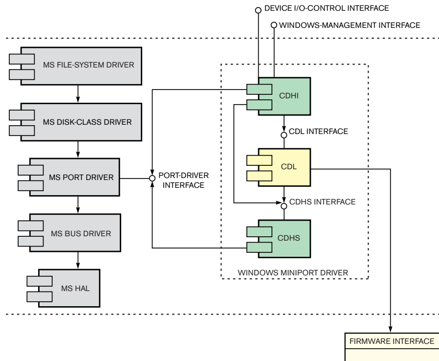
Figure 2 The CDHI- and CDHS-component interface for a miniport in a Windows storage sub-system would have to work with the Microsoft-port-driver interface so that the CDL does not directly interface with the Windows storage stack.
