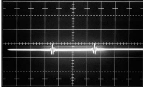
Figure 10 Adding a ferrite bead to the regulator input increases high-frequency losses, dramatically attenuating spikes. (The trace center-screen area is intensified for photographic clarity.)
