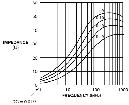
Figure A Impedance versus frequency at various dc-bias currents for a surface-mounted ferrite bead shows essentially zero impedance at dc and low frequency, rising above 50 \Omega depending on frequency and dc current (courtesy Fair-Rite).
