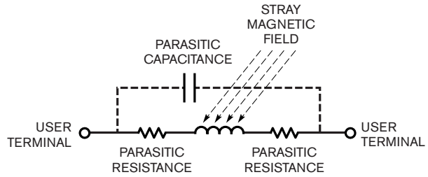
Figure A Some parasitic terms of an inductor show that parasitic resistance decreases voltage, degrading efficiency, and unwanted capacitance permits high-frequency feedthrough. The stray magnetic field induces erroneous inductor current.
